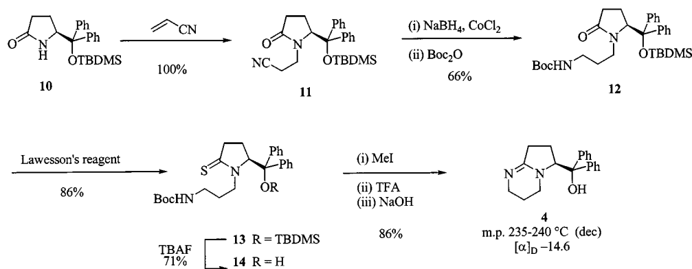
Scheme 1. Synthesis of hydroxyamidine 4
