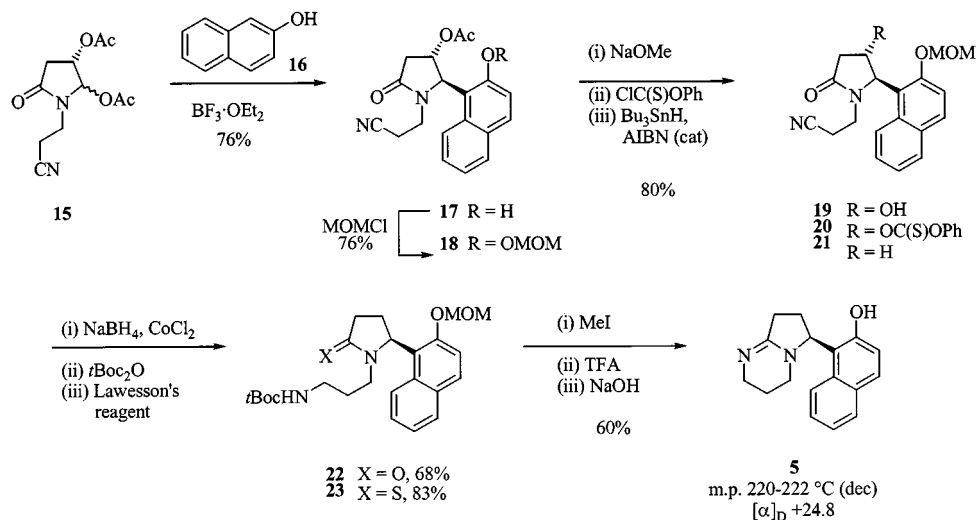
Scheme 2. Synthesis of hydroxyamidine 5
