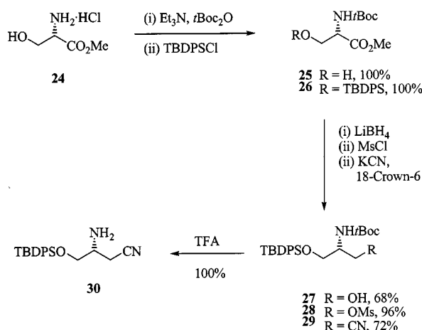
Scheme 3. Synthesis of aminonitrile 30
