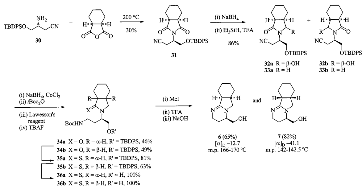
Scheme 4. Synthesis of hydroxyamides 6 and 7
